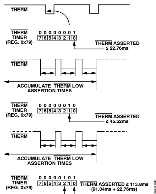
Figure 28. Understanding the THERM Timer
